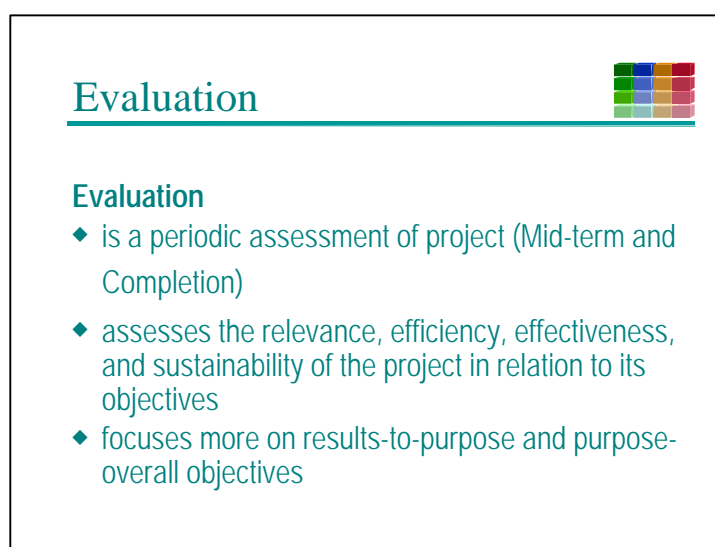
Figure 32: Evaluation
